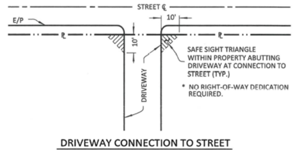
Figure 6 - Diagram demonstrating clear sight triangle requirements by a governing entity (Source: Palm Beach County Department of Engineering & Public Works).
